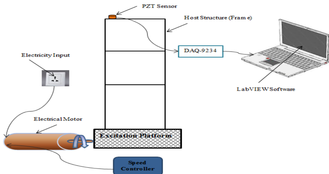
Fig. 2. The Proposed Diagram of Structural Health Monitoring System
